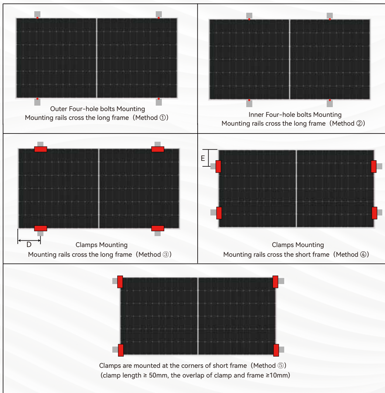
Figure 8 Bifacial Module Installation Position
