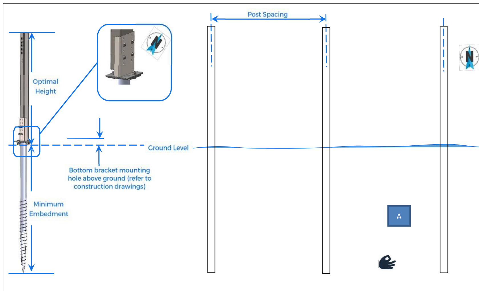
Figure 10: Post installation
