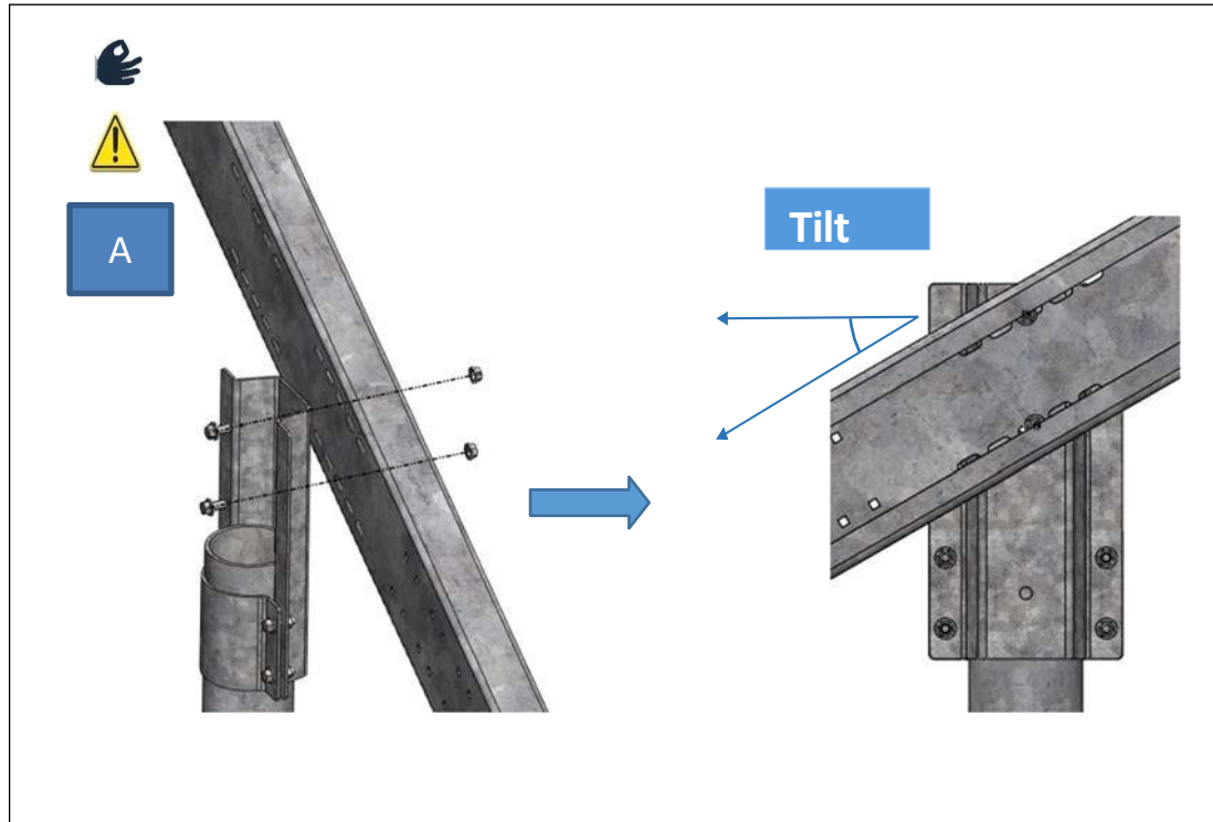
Figure 16: North-South beam Installation
