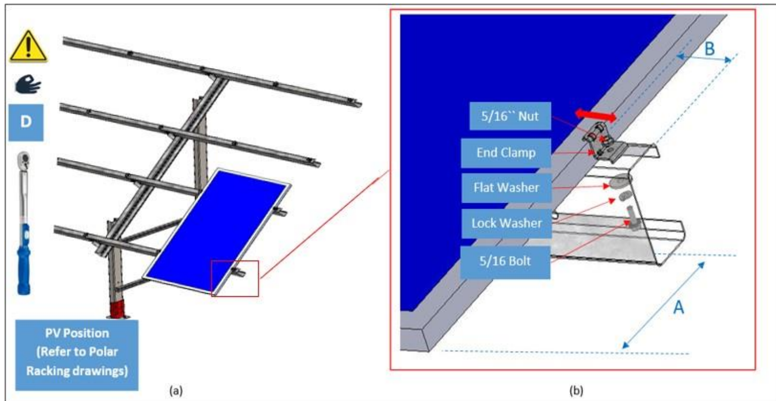
Figure 22: Module to End clamp connection
