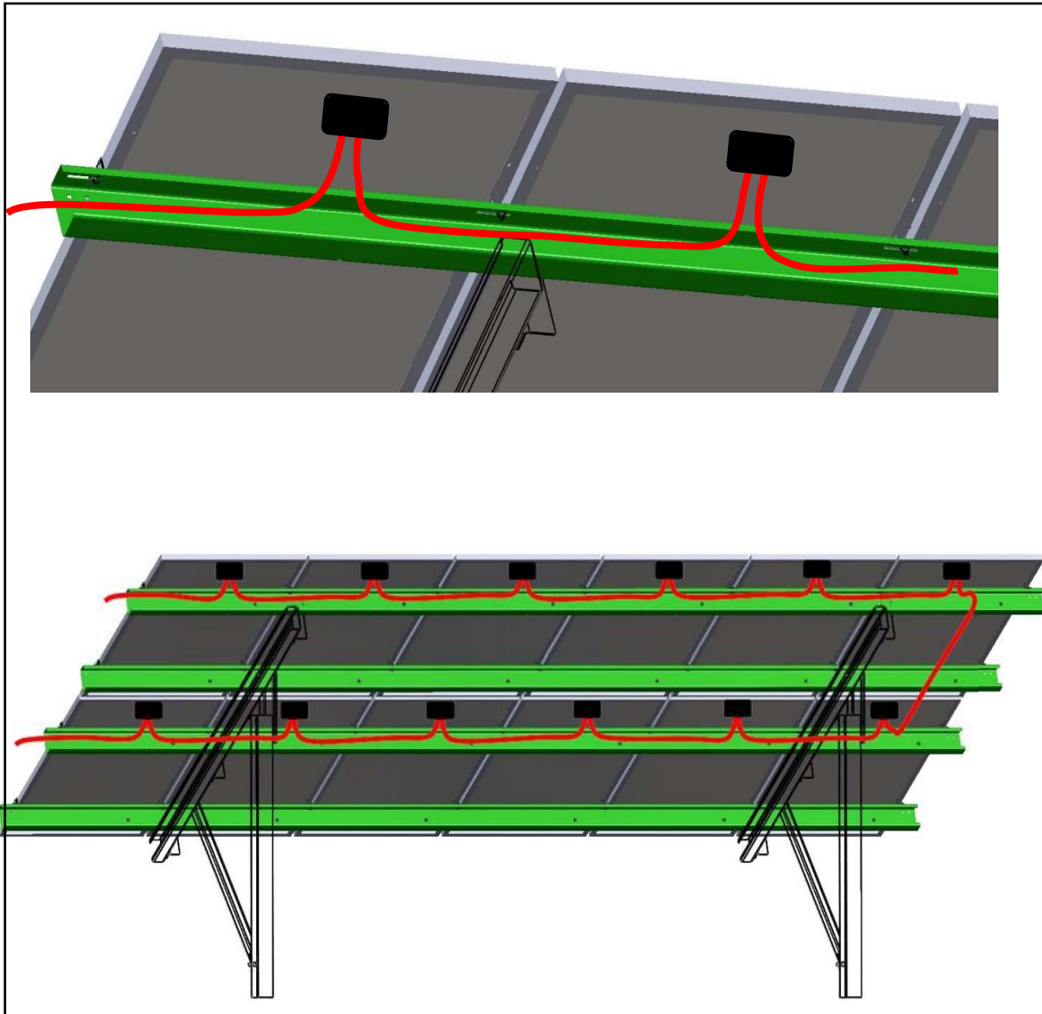
Figure 26: Wire Management
