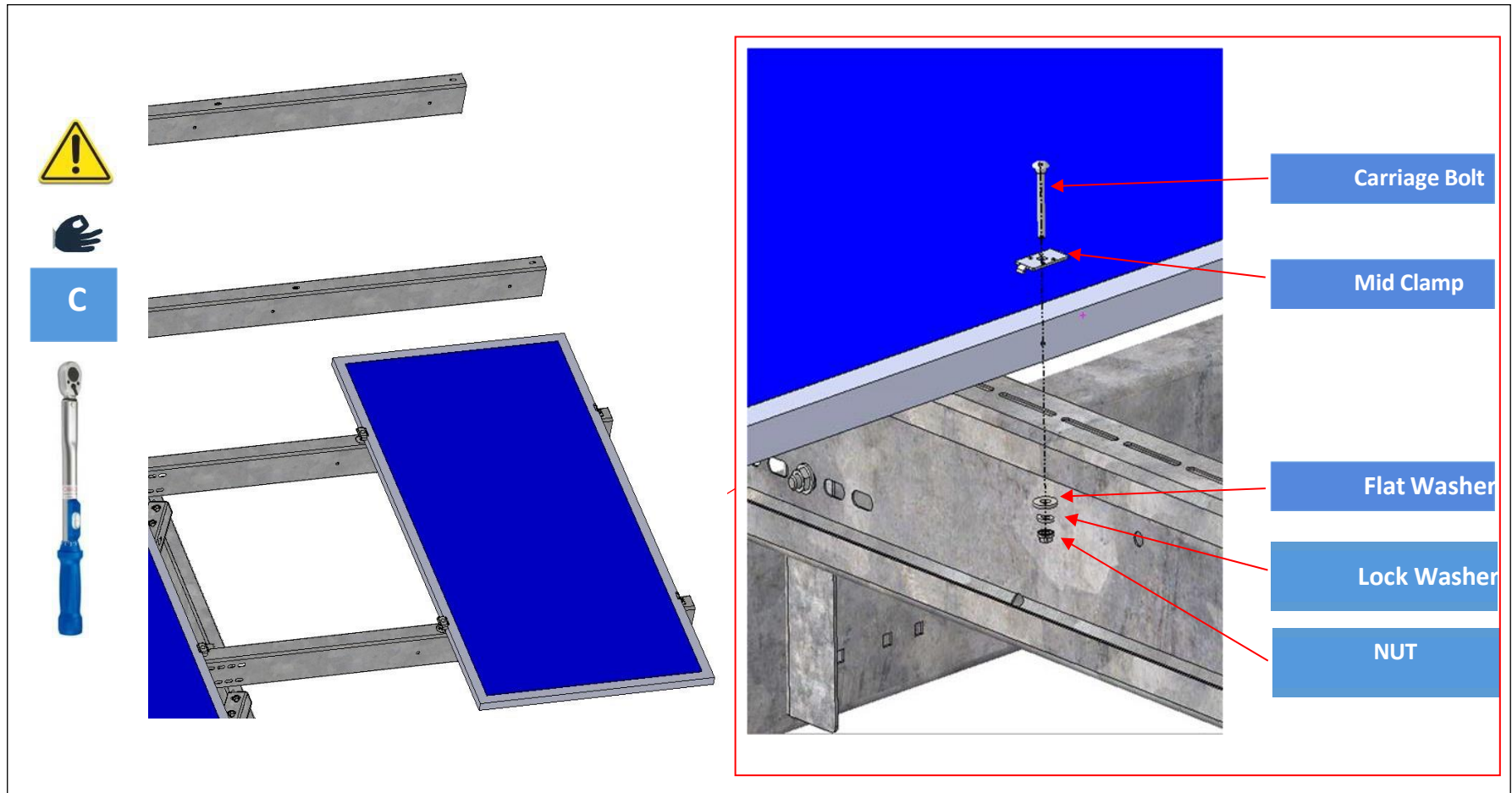
Figure 23: Intermodular connection
