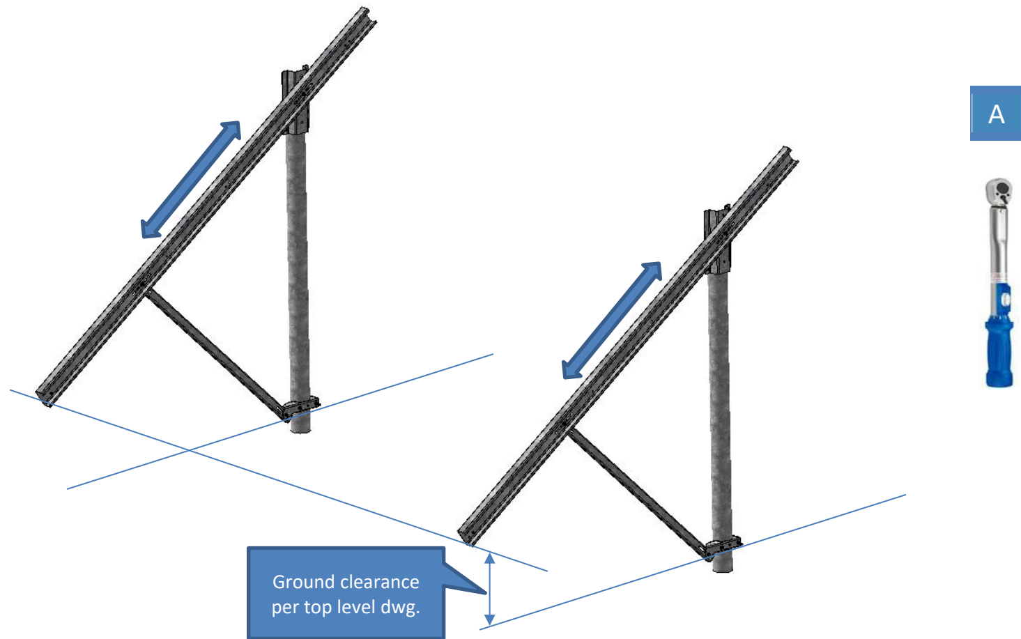
Figure 18: A-Frame alignment
