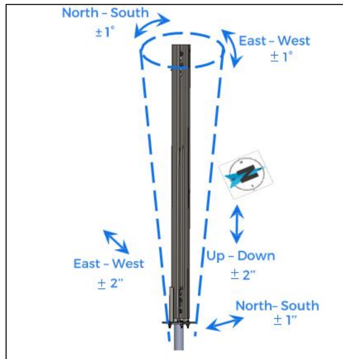
Figure 6: Leg / post installation tolerance
