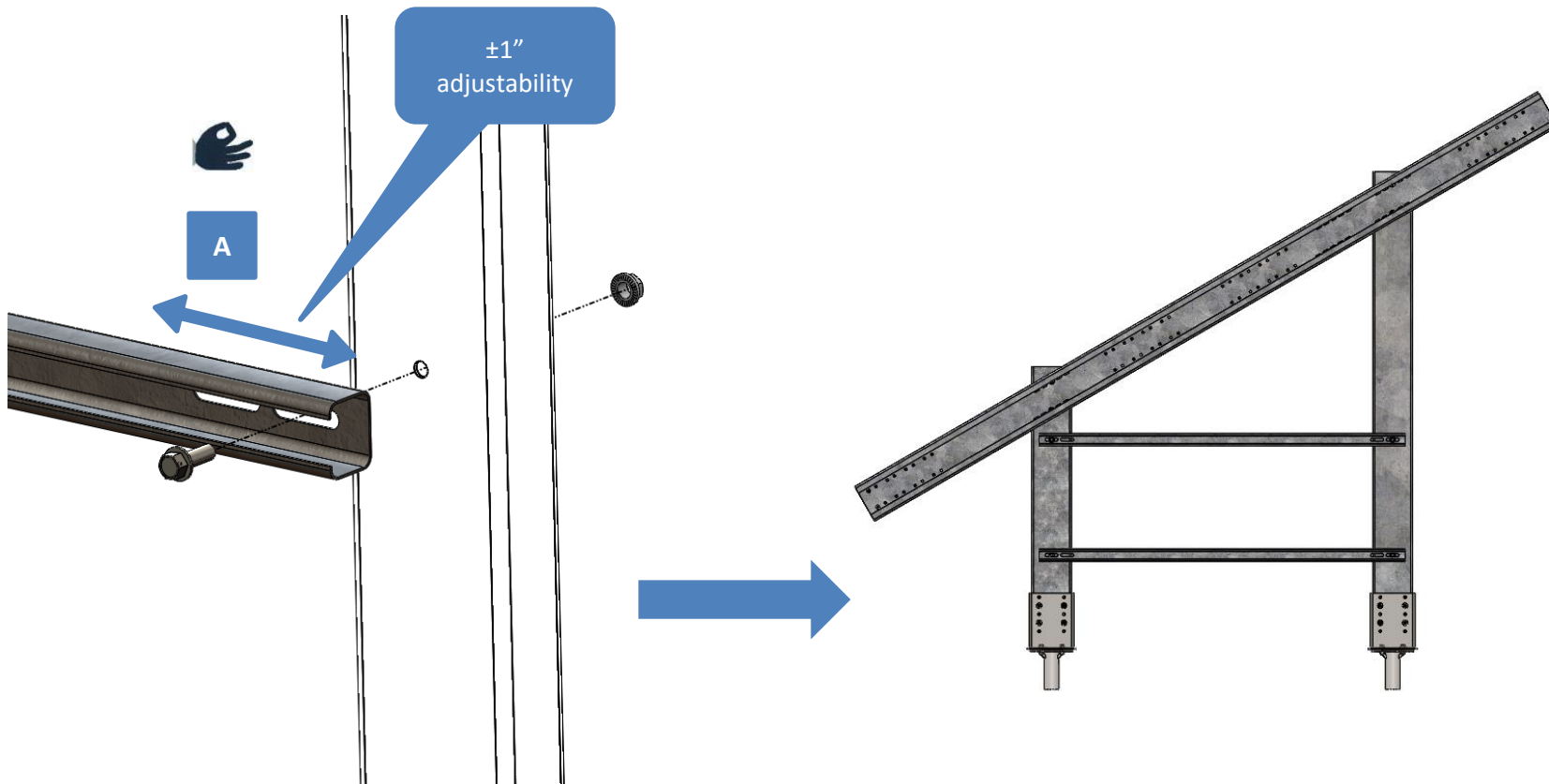
Figure 12: Brace installation
