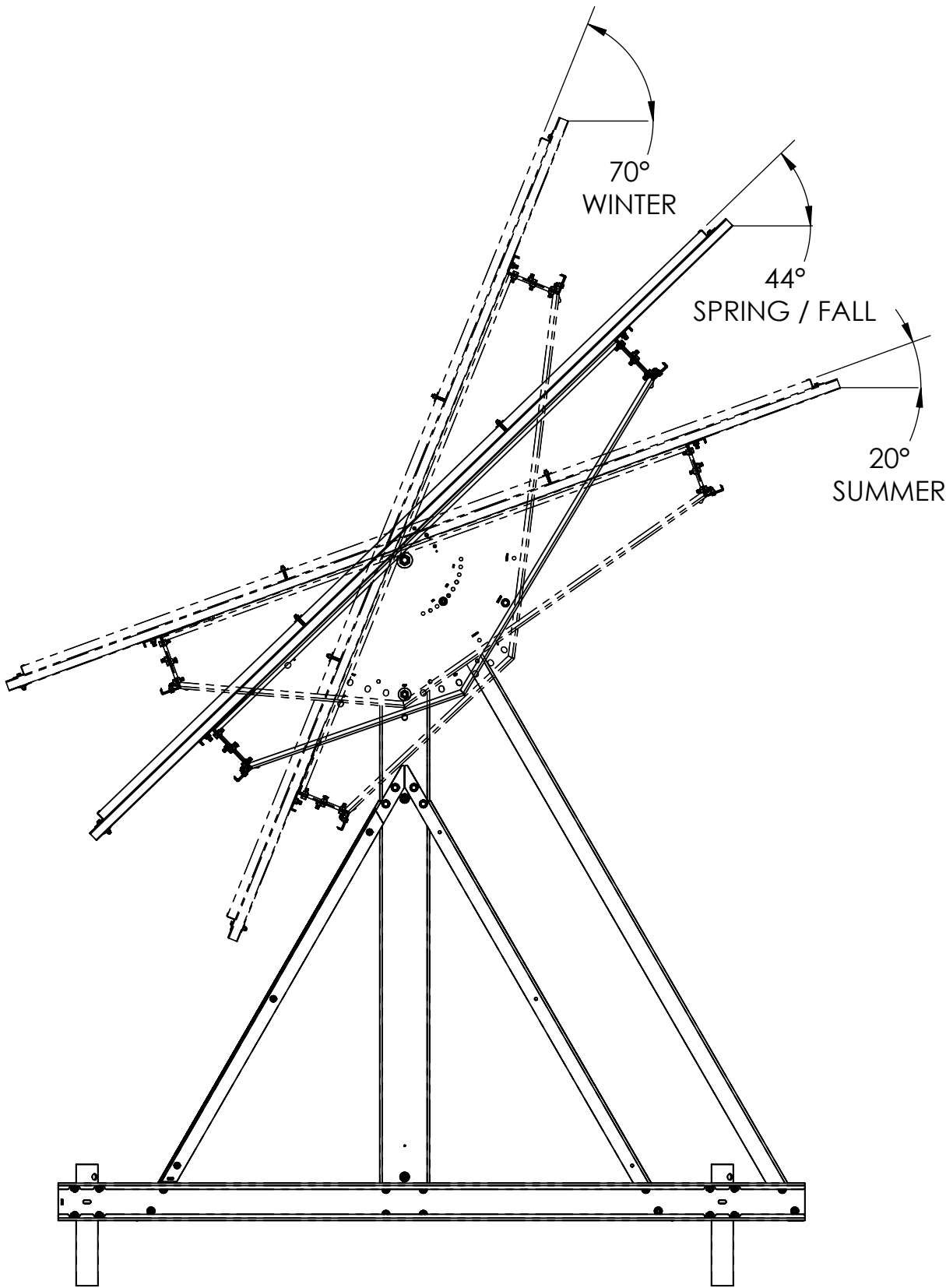
Right Elevation Scale 1:24
