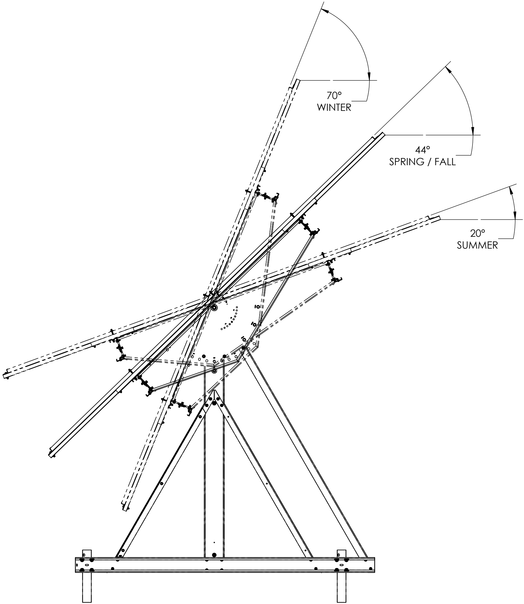
Right Elevation Scale 1:24
