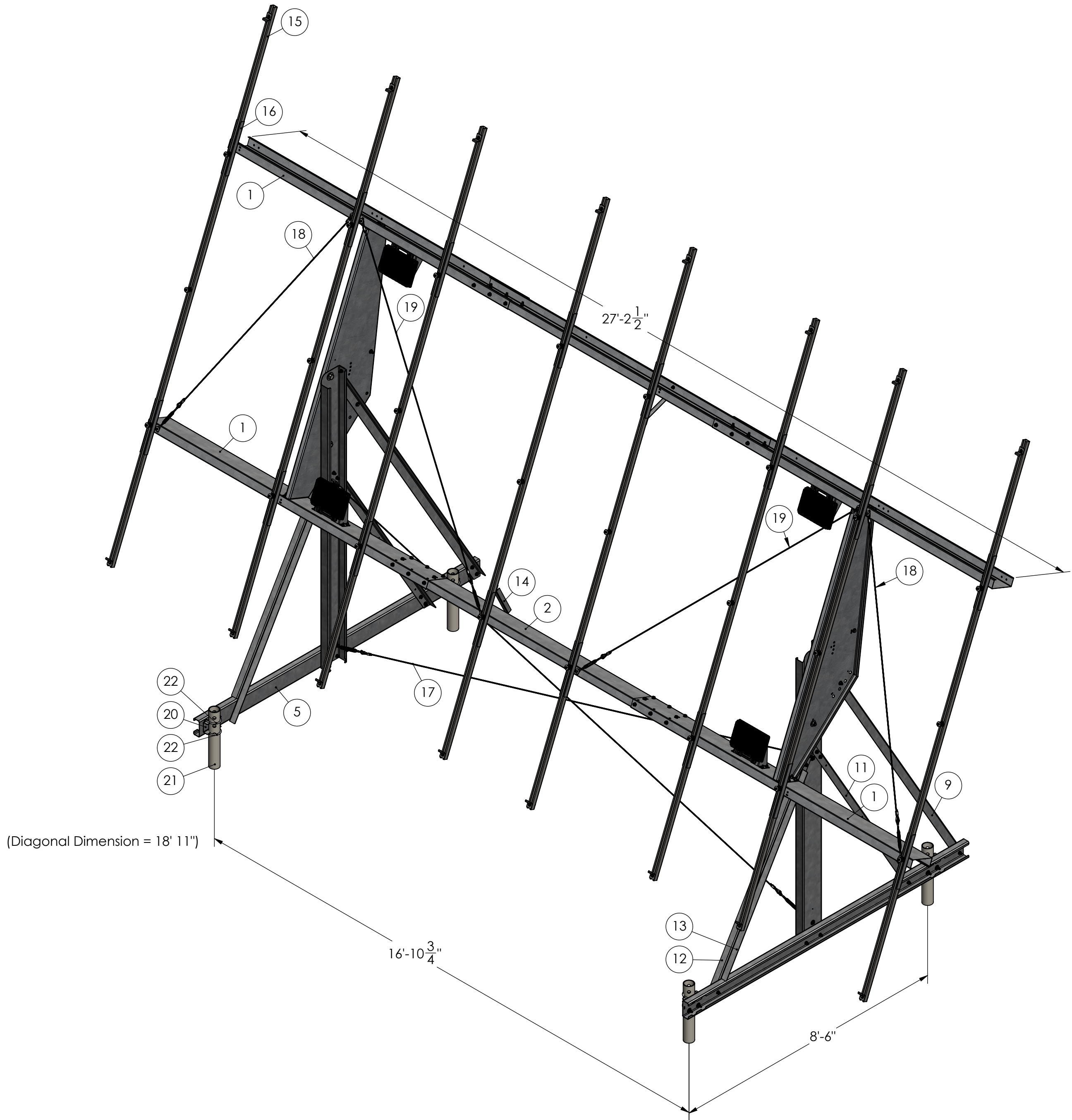
Isometric View Scale 1:24
